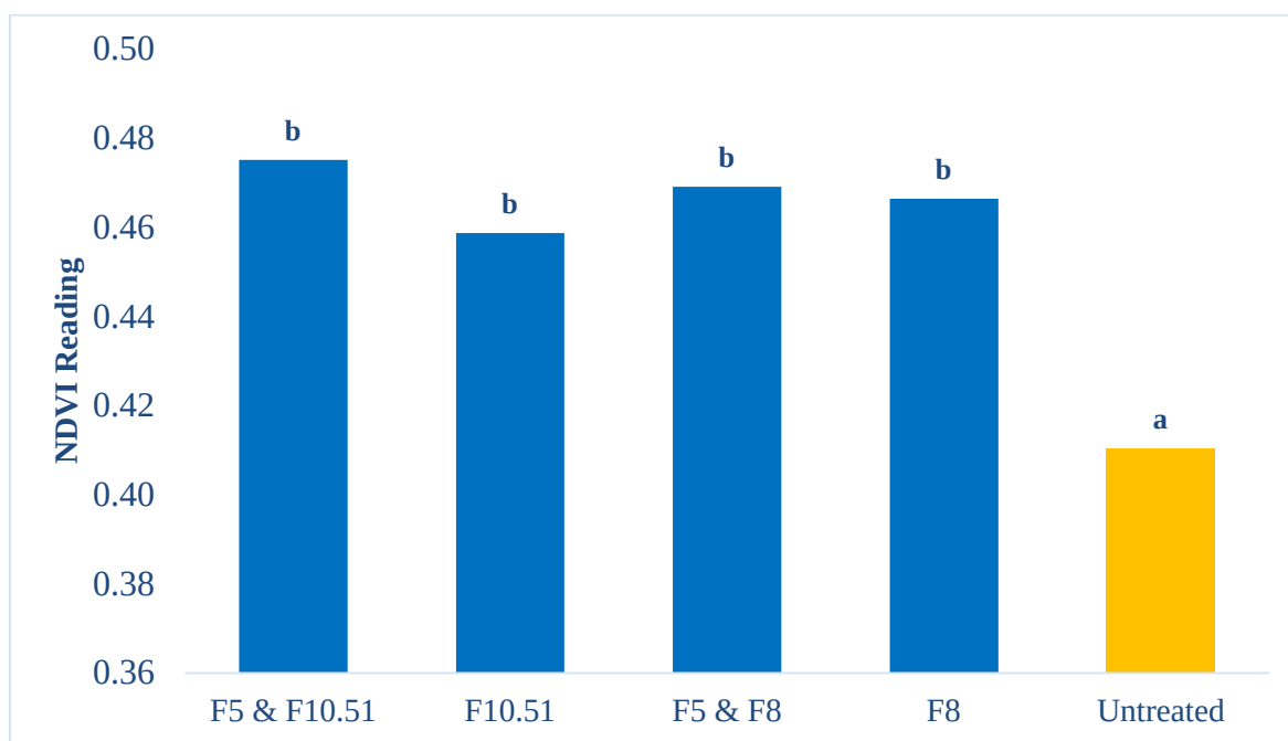
Figure 4. Fungicide program timing had a significant impact on NDVI readings \{P(F)<.0001\} . Timing means followed by the same letter are not significantly different. Means were separated using Fishers Protected LSD ( \alpha=0.05 ).
