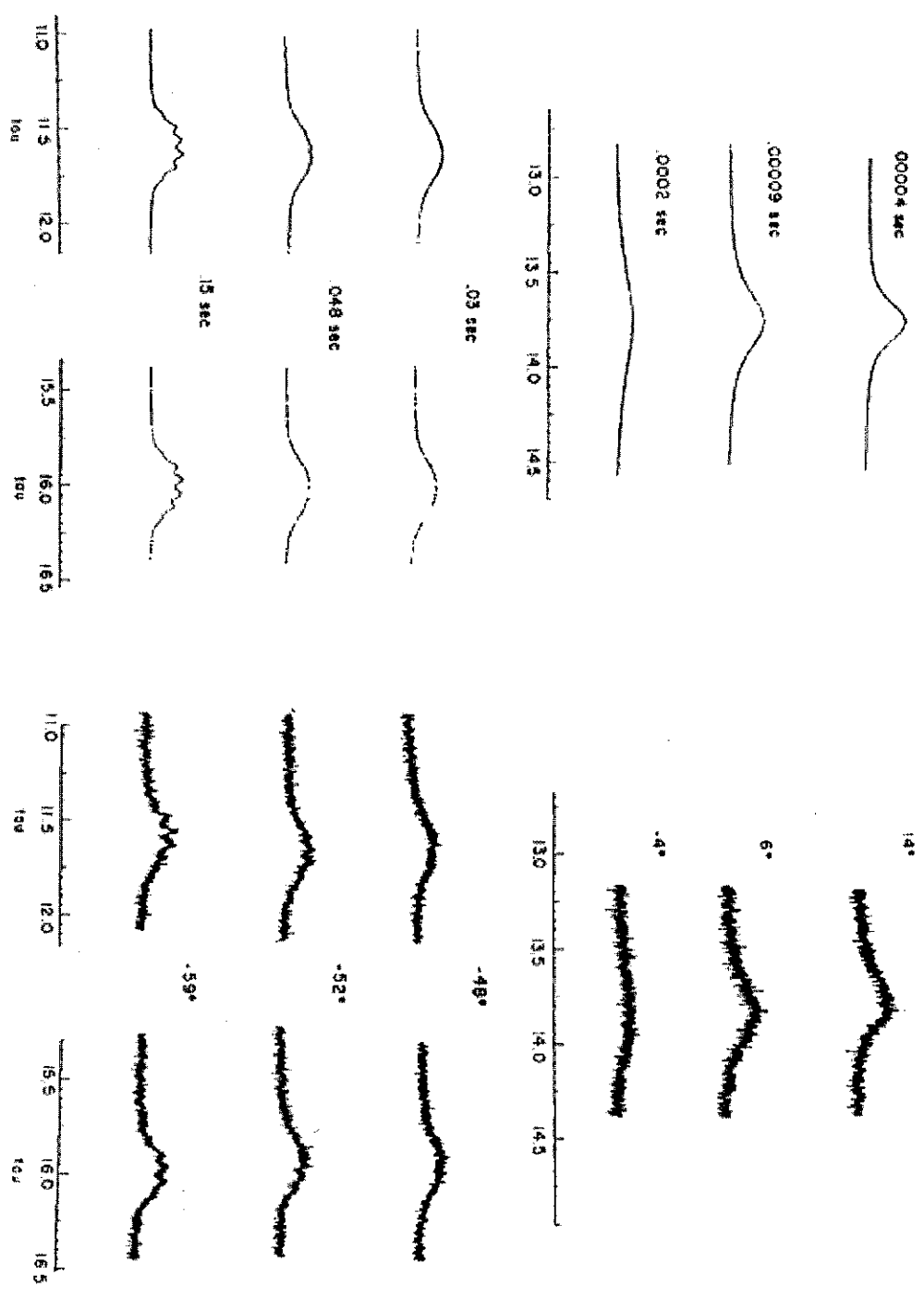
Figure 1. The 100-MHz pmr spectra at several temperatures of the upfield methylene region of [Et_2B(pz)_2]^{73-}CH_2C(Ph)CH_2(CO)_2Mo dissolved in CF_2Cl_2 + CDCl_3 + CH_2Cl_2 (5:5:2).
