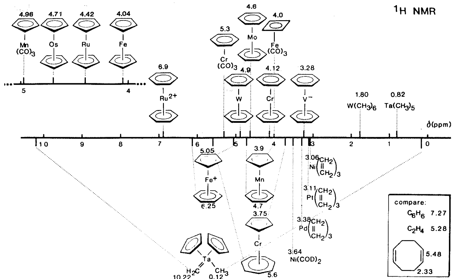
Figure 15-4: \delta^1H values for diamagnetic organotransition-metal compounds.
