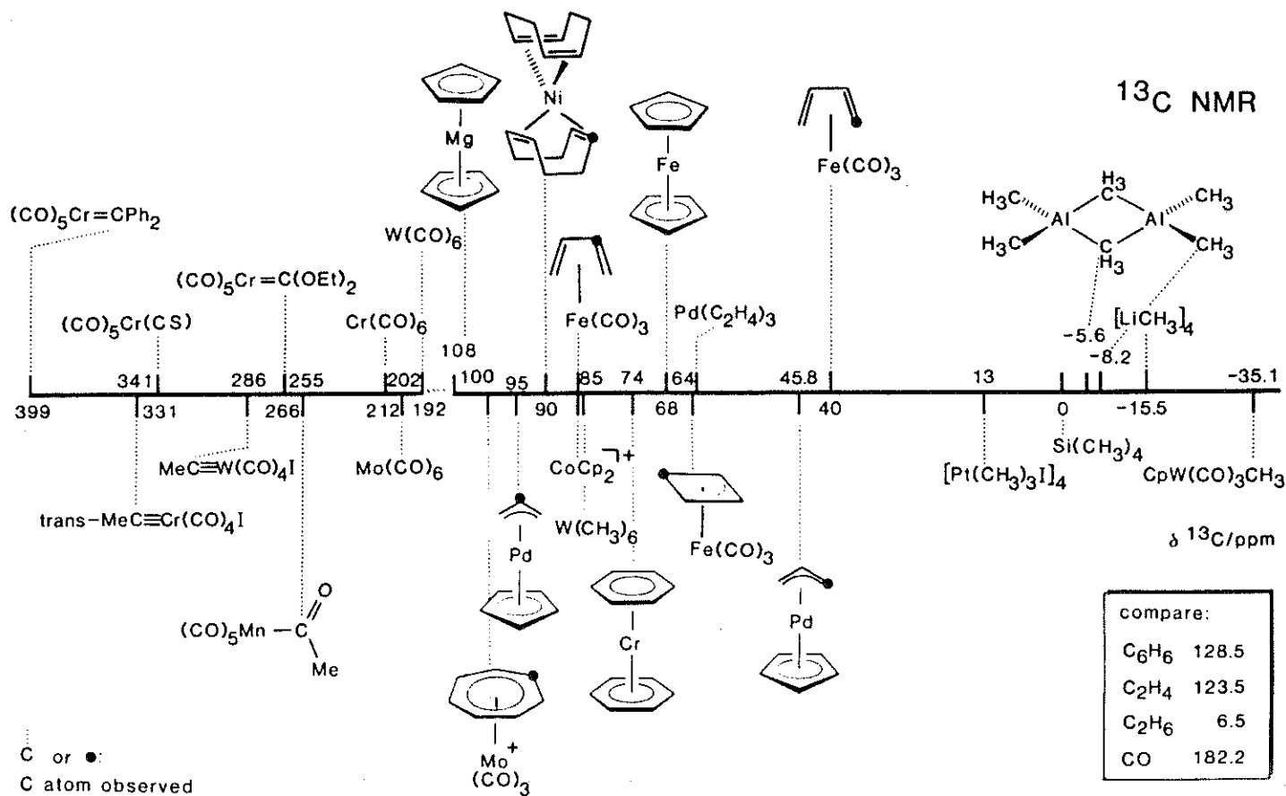
Figure 15-1: Survey of \delta^{13}C values for metal-coordinated carbon atoms of various classes of organometallic compounds.
