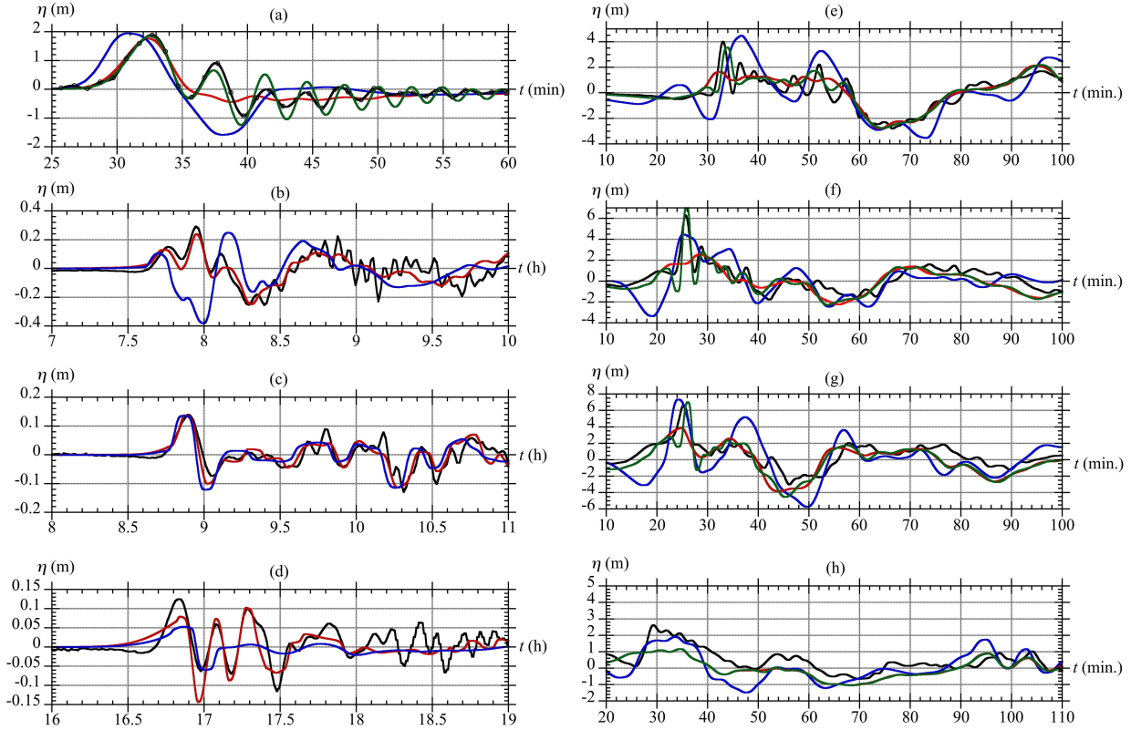
Figure 4 – Comparison between measured surface elevation at DART/GPS buoys (black) [32], and model simulations using UCSB co-seismic source (blue), UA FEM co-seismic source (red), and UA + SMF source (green). DART buoy numbers and lead in model arrival time are : (a) 21418, 0 min (Japan) ; (b) 51407, + 5min (Hawaii) ; (c) 46404, + 6 min (Oregon), (d) 32411, +10 min (Chili). [Model results are offset by the indicated shift to facilitate wave form comparisons.]. GPS buoy locations are (also marked as 4,5,6,9 in Fig. 3) : (e) North Iwate ; (f) Central Iwate ; (g) South Iwate ; (h) South Miyagi (Fukushima). [Note, results in sub-figures (b-d) for far-field DART buoys are for UA and UCSB sources alone as the SMF tsunami would likely not have contributed much to the far-field observations.]
