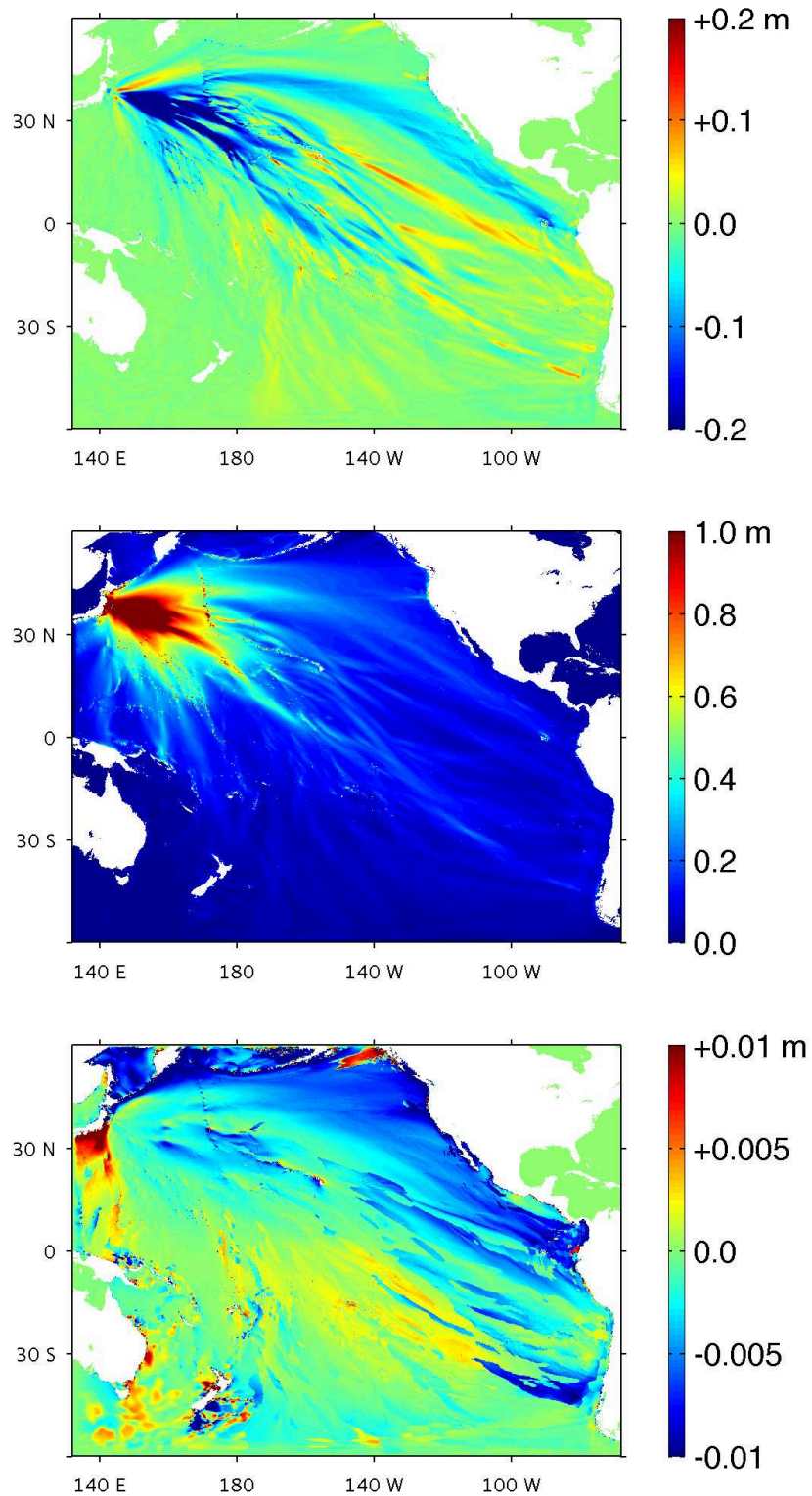
Figure 5 – Envelope of maximum computed wave elevation with FUNWAVE-TVD in spherical ( 2' ) Pacific grid for the UA co-seismic source : (upper panel) difference between maximum wave height envelope with and without dispersion; (center panel) complete result with dispersion and Coriolis terms; (lower panel) difference between maximum wave height envelope with and without Coriolis terms.
