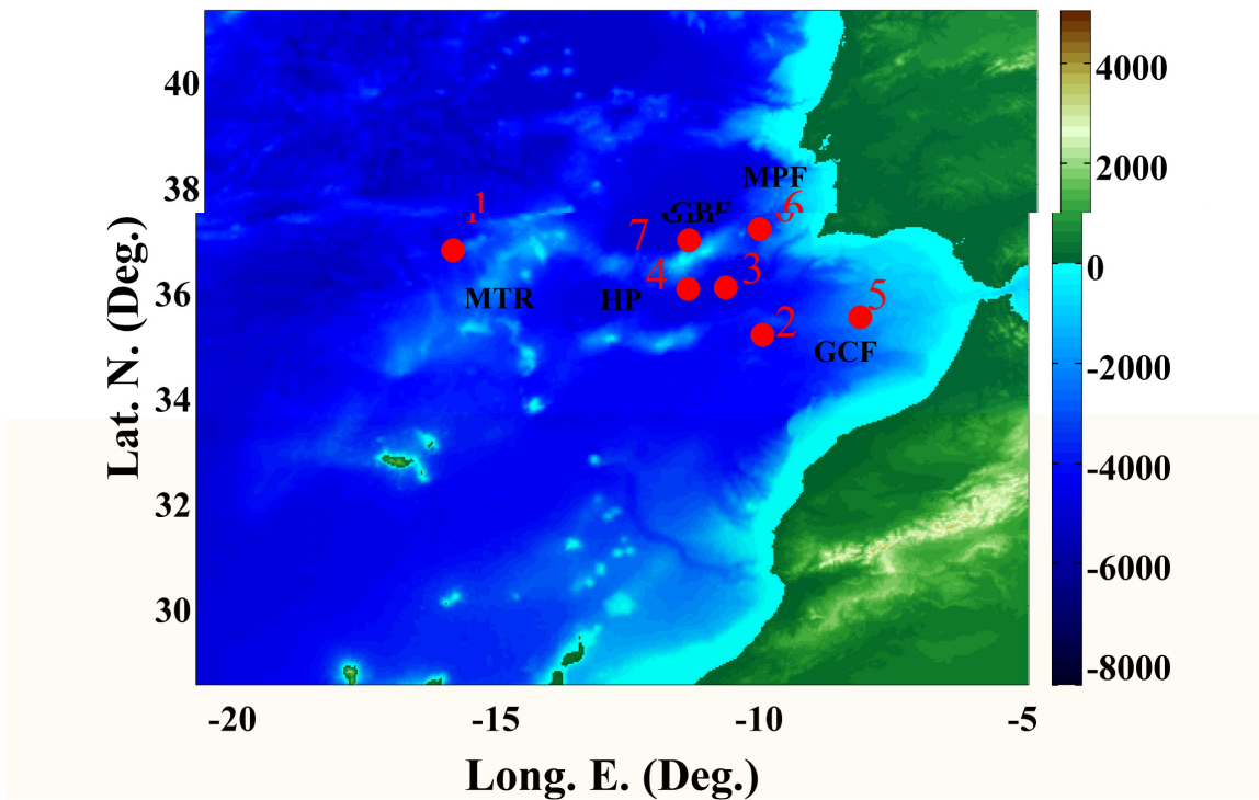
Figure 1: Locations of Lisbon-type co-seismic tsunami sources in the Azores Gibraltar convergence zone. Sources are described in Table 2. MTR refers to the Madeira Tore Rise, HP to the Horseshoe Plain, and GCF, MPF and GBF to the Gulf of Cadiz, the Marques de Plombal, and the Gorringe Bank Faults, respectively.
