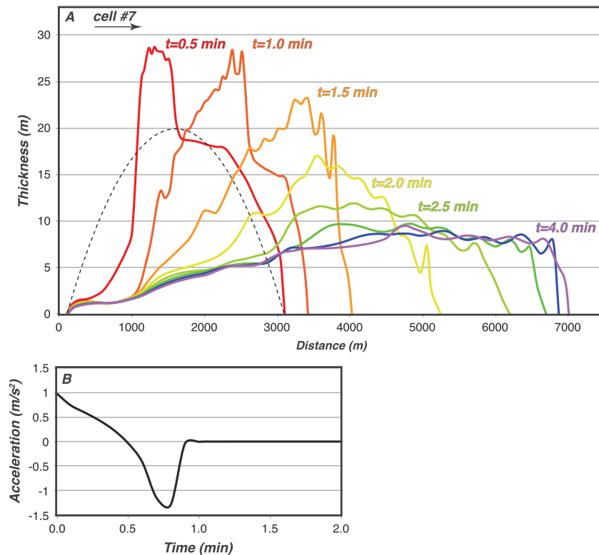
Figure 6. Results from BING modeling of debris flow. (a) Thickness profiles for the first 4 min of movement are shown at 0.5 min increments. The initial thickness profile is parabolic, as indicated by the black dashed line. (b) The acceleration time history for cell #7 is shown, which is located 420 m from the back of the slide. The horizontal downslope movement of cell #7 is indicated by the arrow in Figure 6a.
