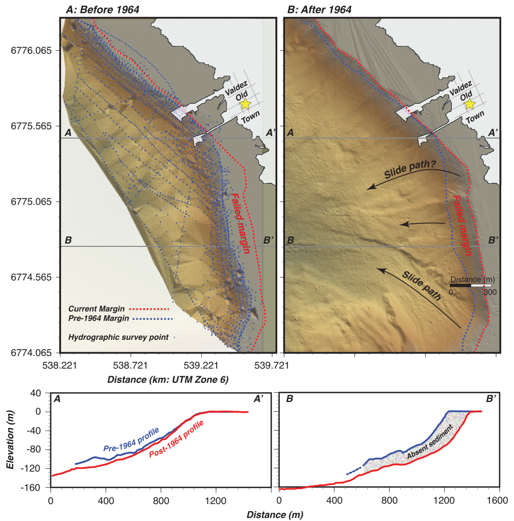
Figure 3. (a) A hydrographic survey conducted in 1957 gives the approximate preearthquake shape of the fjord margin near Valdez old town and the location of the slope edge. (b) Multibeam bathymetry data show the postlandslide configuration, with parts of the slope edge recessed ~150 m east of the preearthquake location, mostly south of Valdez old town (labeled “Failed margin”). Cross sections A-A’ and B-B’ show differences between the two surveys where the margin is largely unchanged and where significant submarine landsliding took place, respectively.
