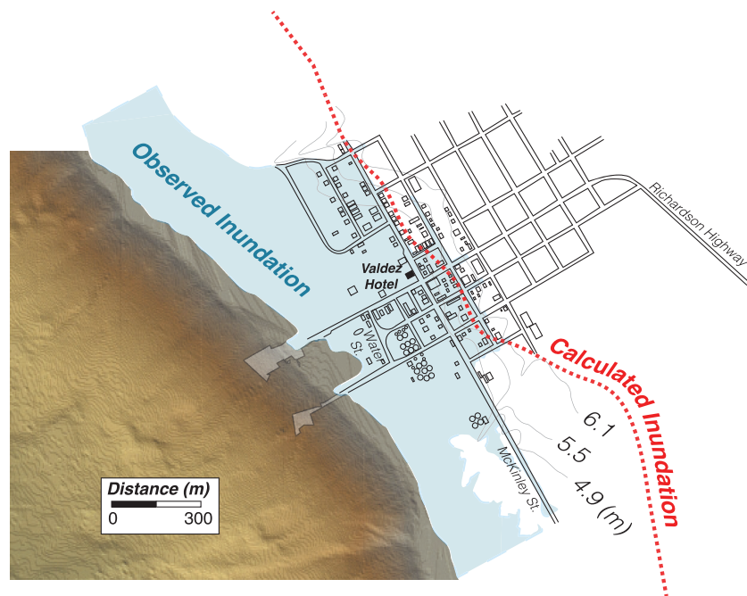
Figure 10. Comparison of observed tsunami inundation (blue shading) [Wilson and Tørum, 1971] in Valdez old town with calculated maximum inundation (red dashed line) from the delta-front slide source. Postearthquake elevation contours are shown that imply that the observed water height reached 6.1 m above mean sea level. The tsunami modeling used a smoother version of the topography to make calculations possible. However, a fairly close match between observed and calculated runup heights was achieved.
