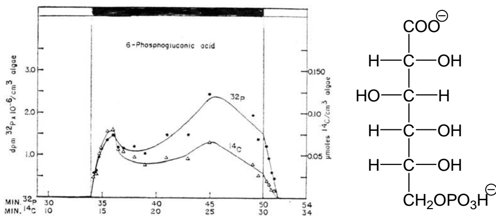
Figure 2. The effect of light and dark on the amount of labeled 6-phosphogluconate in algal cells. Conditions as described in Figure 1.
