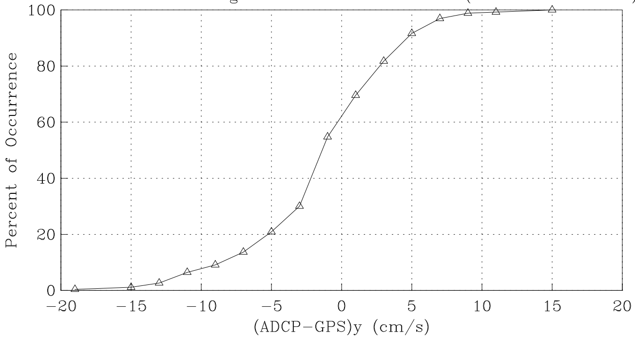
SBI-2004 Fall Mooring Cruise ADCP Calibration (09-12-2004 amue)
