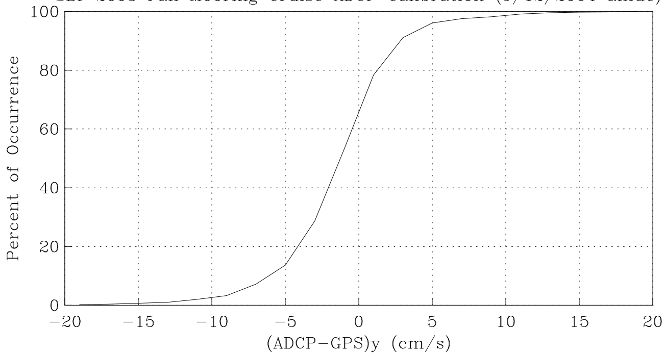
SBI-2003 Fall Mooring Cruise ADCP Calibration (9/12/2004 amue)
