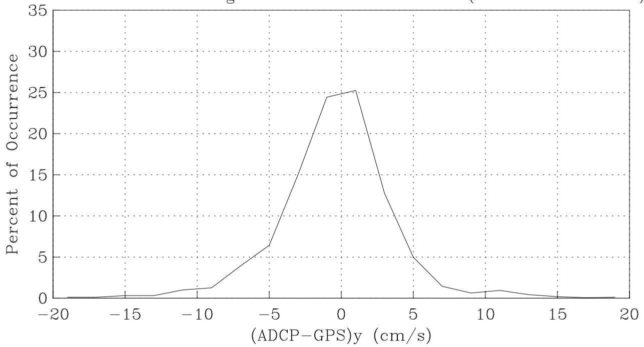
SBI-2003 Fall Mooring Cruise ADCP Calibration (09-12-2004 amue)
