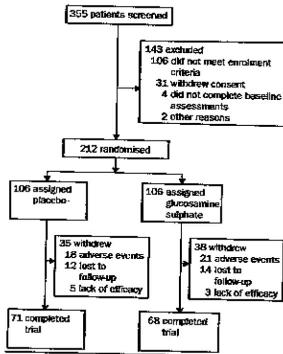
Figure 1: Trial profile
